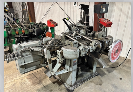
Nilson Model S2F Four-Slide Machine
