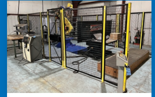
Robotic Wire Grid Welder
