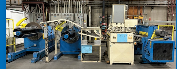
48" x 10,000 Lb. Dual Uncoiler Cut-to-Length Line
