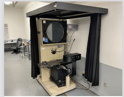
20" Dorsey Optical Comparator with Acu-Rite DRO
